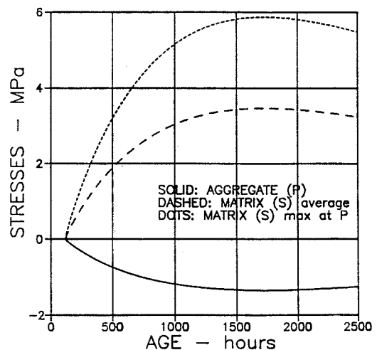
Figure 24. HETEK-concrete exposed to drying at RH = 50 % from the age of 5 days. All data are averages.
