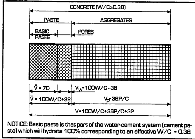
Figure 7. Volume composition of concrete with W/C \geq 0.38 . Composite system I: Paste = Basic paste + pores. Composite system II: Concrete = Paste + aggregates. The following abbreviations are used: W , C , and P are weights of water, cement, and aggregates respectively. V means volume. Subscripts W and P refer to water and aggregate respectively.
