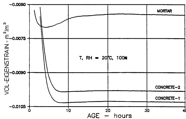
Figure 18b. Blow-up of Figure 18a at low ages. Age at start of solidification t_s is defined at first positive derivative of shrinkage graph. Mortar starts solidifying at t_s \approx 5 hours, concrete at t_s \approx 10 hours.
