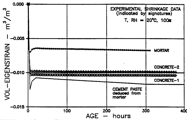
Figure 18a. Symbols: Measured auto-shrinkage of mortar and concrete. Solid line: Cement paste auto-shrinkage deduced from mortar tests.
