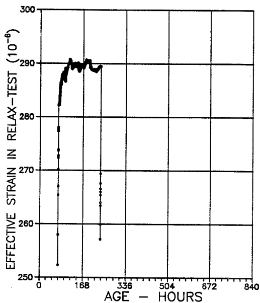
Figure 28. Effective strain in relaxation experiment (cleared with respect to shrinkage).
