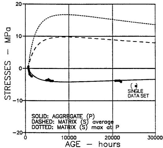
Figure 26. Nielsen-concrete (LL3) exposed to drying at RH = 60 % from the age of 28 days. All predicted data are averages.
