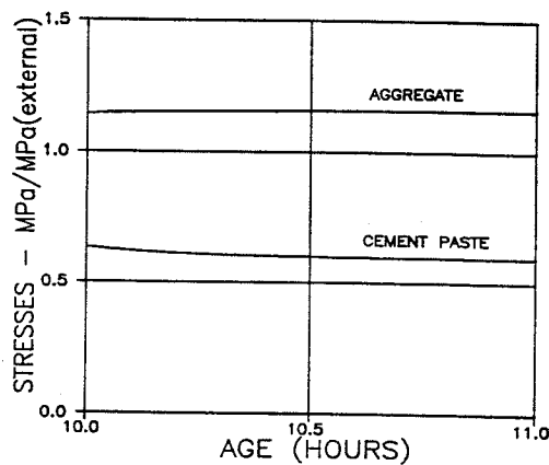
Figure 27. Stresses in HETEK-concrete loaded with 1 MPa at the age of 10 hours. Stresses do not change very much from the age of 11 hours.
