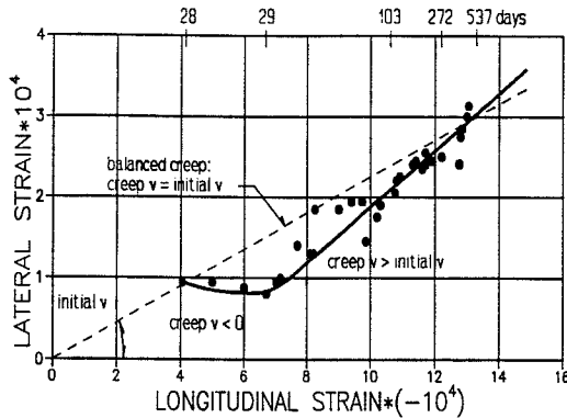
Figure 5. Lateral creep versus longitudinal creep of a granite concrete.
