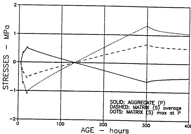
Figure 20. Internal stresses in HETEK-mortar caused by auto-shrinkage. Start of solidification assumed at t = 5 h.
