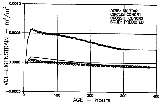
Figure 21. Lower data: Shrinkage difference of concrete in period, age 10 hours (start of concrete solidification) to t . Concretes 1 and 2 almost coincide.
