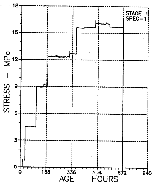
Figure 10. DTI-test st1-spl: Load applied.
