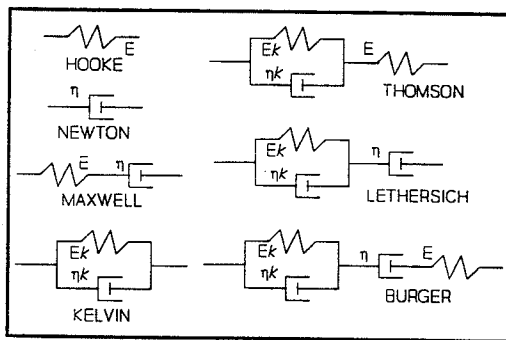
Figure 3. Mechanical analogies to linear viscoelastic materials.
