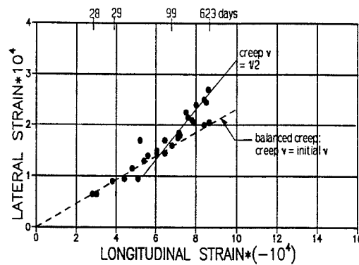
Figure 6. Lateral creep versus longitudinal creep of a basalt concrete.
