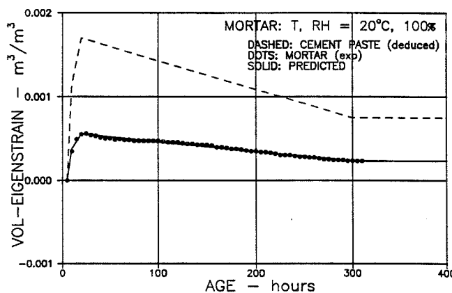
Figure 19. Shrinkage difference of mortar in period, t_s = 5 hours (start of solidification) to t .
