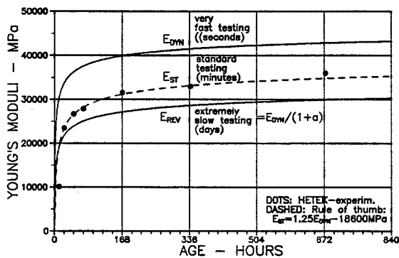
Figure 9. Stiffness moduli for HETEK-concrete defined in this section.
