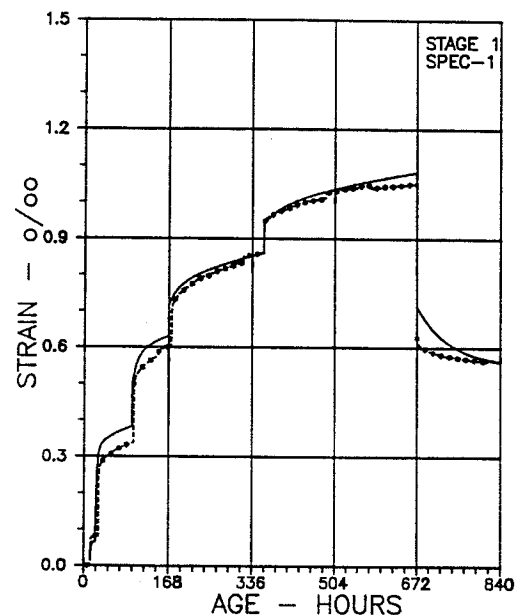
Figure 11. DTI-test st1-spl: Creep strain observed.
