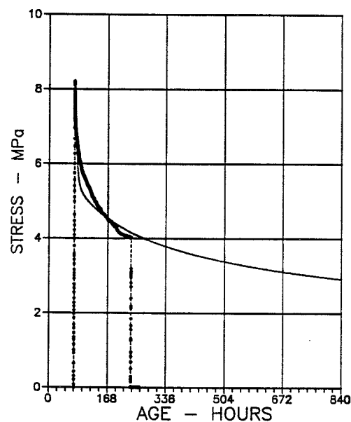
Figure 29. Relaxation: Experimental (partly coinciding dots) and predicted (solid line) as explained in main text.
