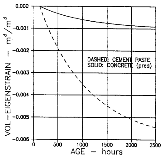
Figure 23. HETEK-concrete exposed to drying at RH = 50 % from the age of 5 days. All data are averages.
