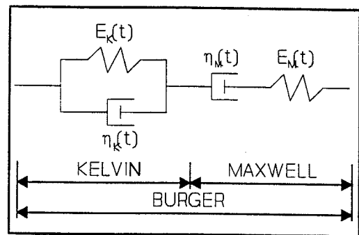
Figure 4. Burger model of aging linear viscoelastic material.
