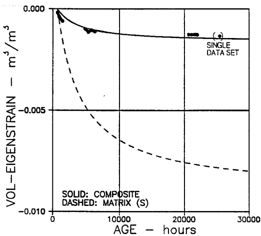
Figure 25. Nielsen-concrete (LL3) exposed to drying at RH = 60 % from the age of 28 days. All predicted data are averages.
