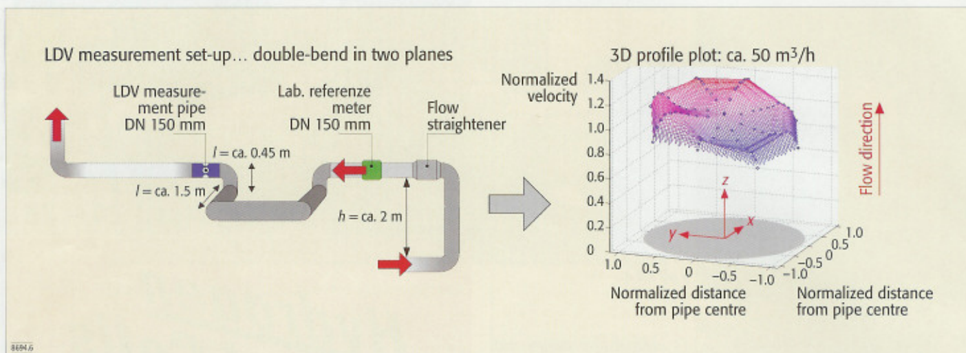
Figure 6. The installation of a 90° double-bend in 2 planes, and the resulting 3D LDV profile plot.
