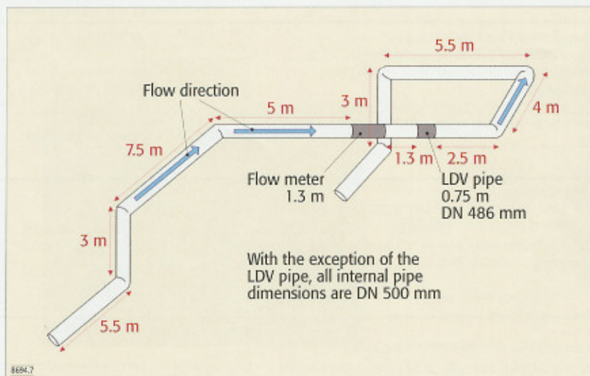
Figure 7a. Installation diagram of the on-site calibration of a 500 mm flow meter
