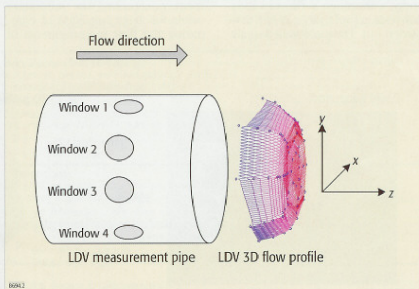
Figure 2. The generation of a 3D LDV flow profile from measuring point velocities across several pipe diameters
