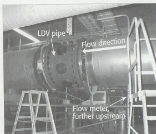
Figure 8b. Photo of the installation
