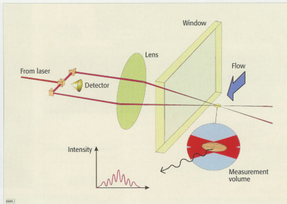
Figure 1. Simple illustration of the Laser Doppler Velocimetry (LDV) principle
