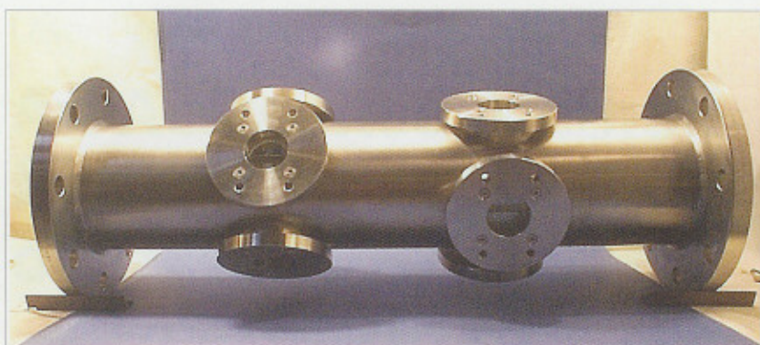
Figure 3. Window construction for laboratory use
