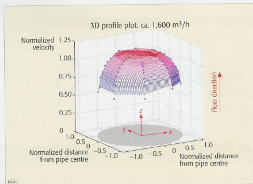
Figure 9. A 3D LDV profile plot from calibration of a 1000 mm flow meter, showing a fully-developed flow
