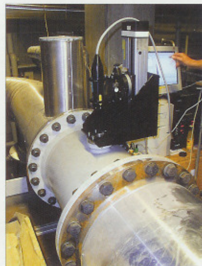
Figure 7b. Photo of the installation
