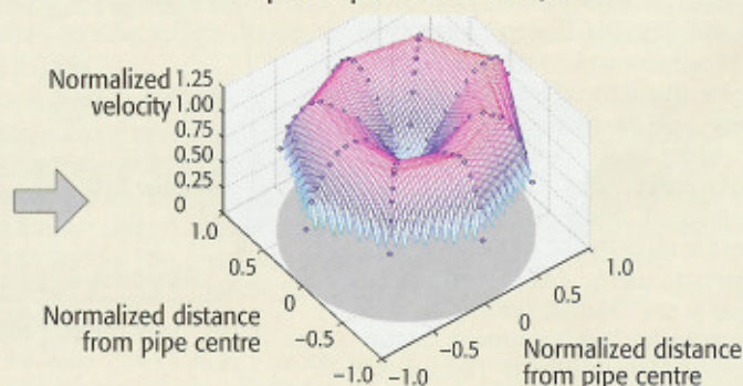
3D profile plot: ca. 100 m³/h
