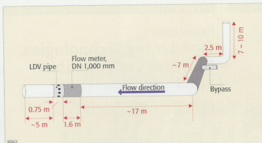
Figure 8a. Installation diagram of the on-site calibration of a 1000 mm flow meter
