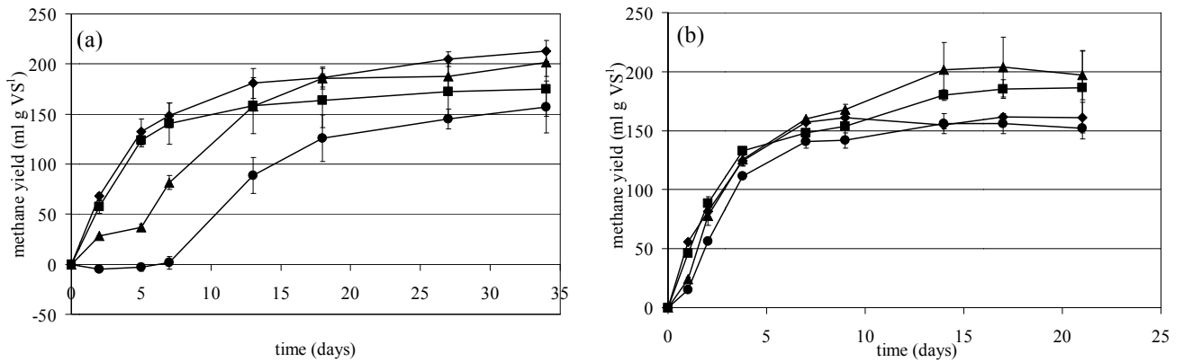
Fig. 3.7 Toxicity tests of Ulva lactuca . Batch vials containing inoculum from a thermophilic CSTR treating cattle manure were added various concentrations ( \blacklozenge : 2.5 \text{ g VS l}^{-1} ; \blacksquare : 5.0 \text{ g VS l}^{-1} ; \blacktriangle : 10.0 \text{ g VS l}^{-1} ; \bullet : 20.0 \text{ g VS l}^{-1} ) of wet and dry Ulva lactuca and incubated at 53^\circ\text{C} . a) Wet Ulva lactuca b) Dry Ulva lactuca . As seen, the biogas process was more sensitive towards wet algae compared to dry algae.
