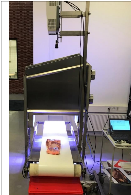
Figure 2. The pilot setup including DynaCQ sensor, projector and RGB camera
